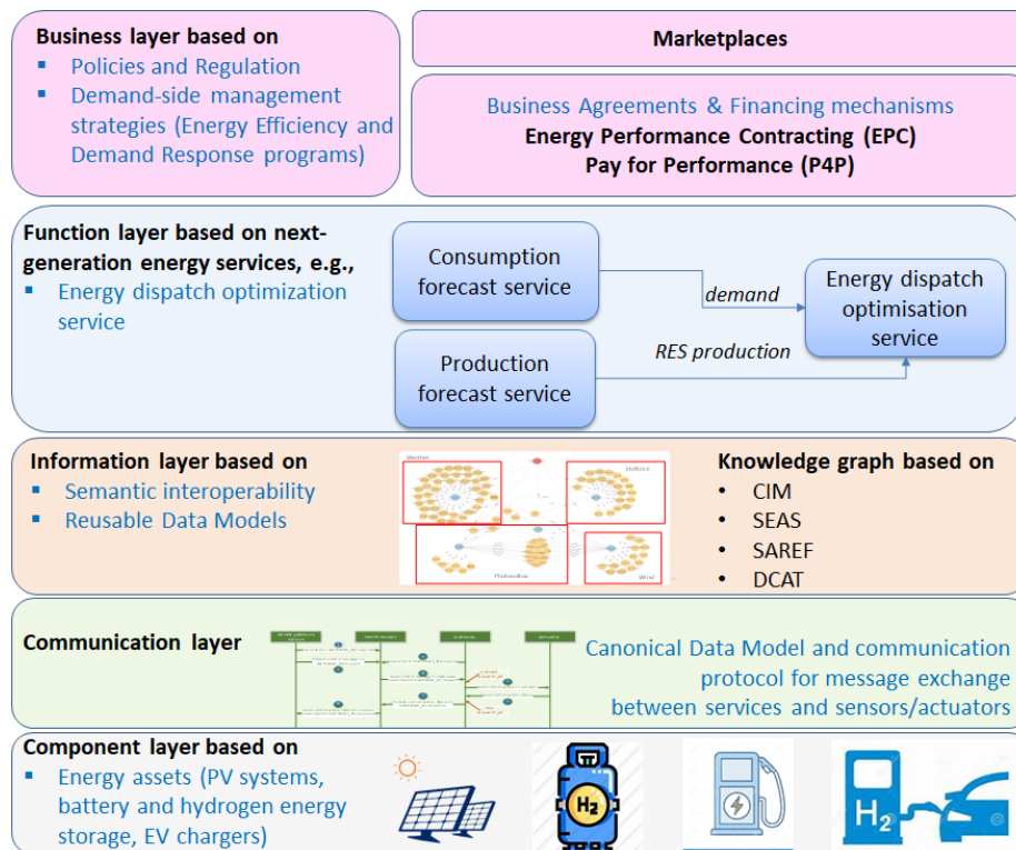
Figure 1: Platform architecture (SGAM interoperability layers)
