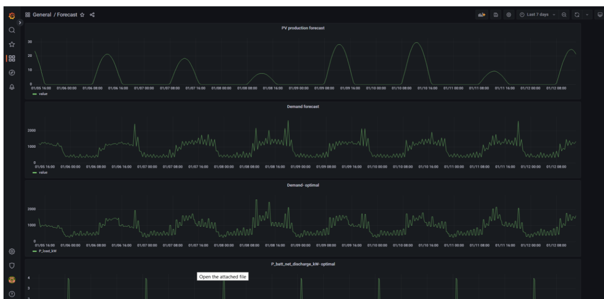
Figure 3: PV production forecast, demand forecast and optimal demand profiles (visualized in Grafana web interface)
