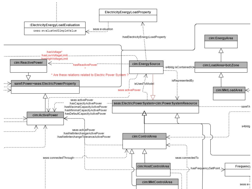
Figure 1. Applying the CIM standard.
