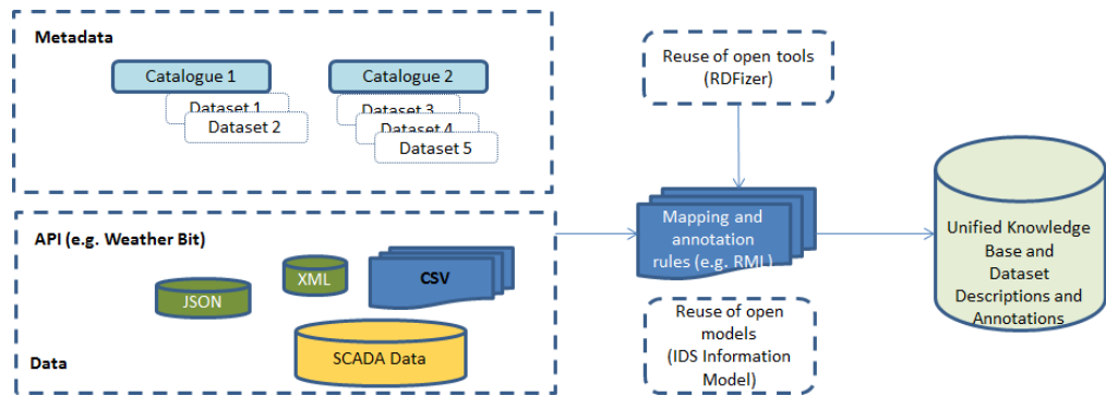
Figure 4. Data harmonization pipeline.
