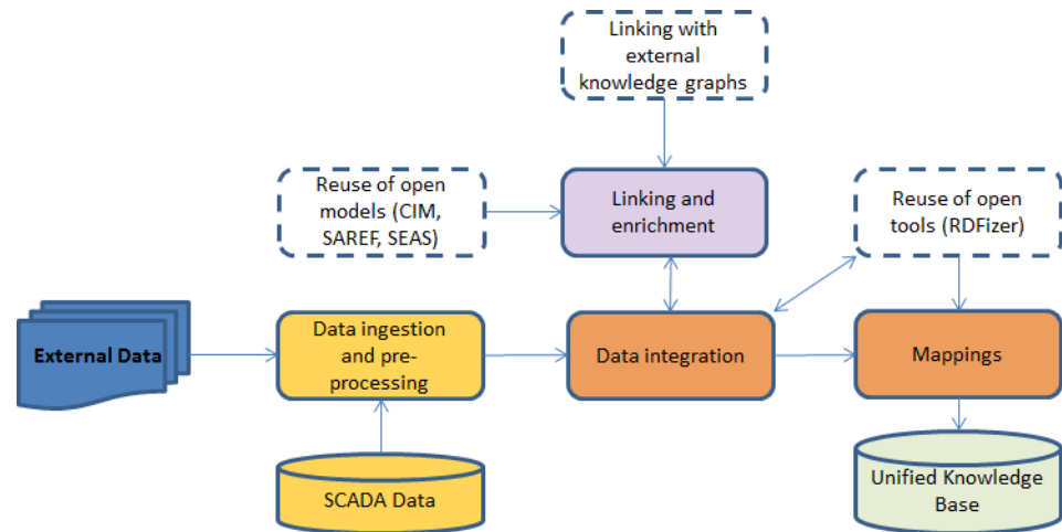
Figure 3. Unified knowledge graph creation process.
