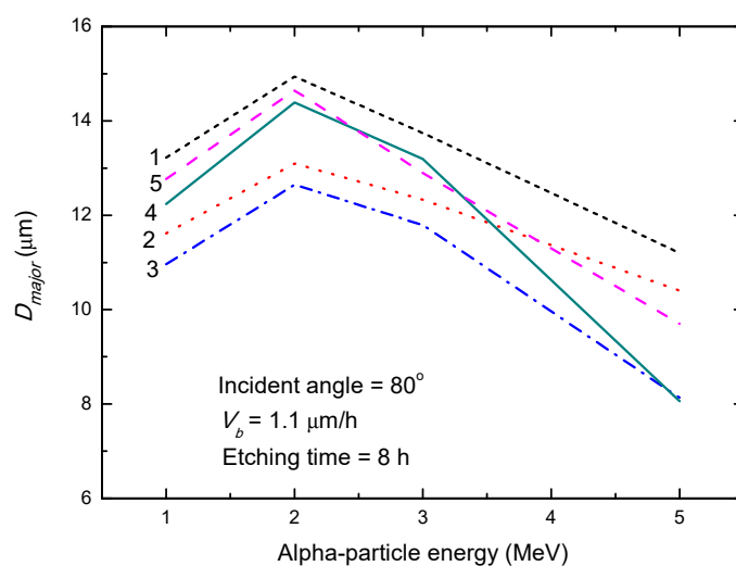
Figure 1. Relationship between the major-axis length ( D_{major} ) of the track opening in the CR-39 detector and the alpha-particle energy for the incident angle of 80^\circ for the five V functions implemented in the revised TRACK_TEST program. The experimental conditions are given in Figure. 1: V function No. 1 [13], 2: V function No. 2 [14], 3: V function No. 3 [15], 4: V function No. 4 [19] and 5: V function No. 5 [20]. Functions 4 and 5 were newly added in the revised TRACK_TEST program.
