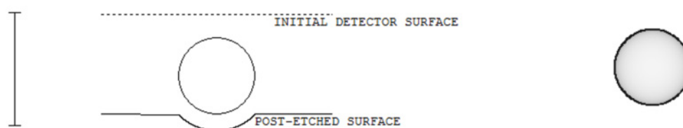
Figure 4. Simulated results obtained by the revised TRACK_VISION program corresponding to those alpha-particle tracks developed on an irradiated and etched Makrofol detector shown in Figure 3. Left panel: track profile and track opening (the latter being a circle due to normal incidence), together with the position of the detector surface before and after etching. Right panel: optical track appearance, which consists of a wide, dark ring and a bright area at the track center. Vertical left bar represents 34 \mu\text{m} .
