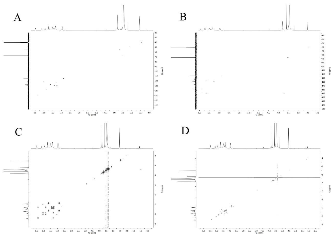
Slika P71. HSQC (A), HMBC (B), COSY (C) i NOESY (D) 2D NMR spektri kompleksa 4-Se .
