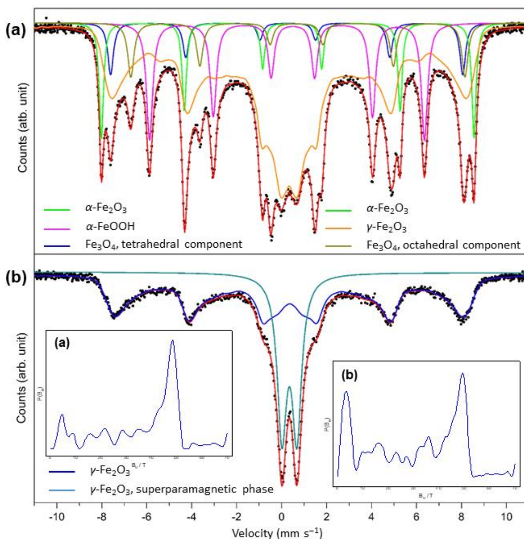
Figure 19. ^{57}\text{Fe} Mössbauer spectra of (a) \text{MAG}_{\text{MW}} and (b) \text{MAG}_{\text{MW-CLI}} samples recorded at room temperature ( \bullet stands for experimentally obtained data). The insets show the B_{\text{hf}} distribution.
