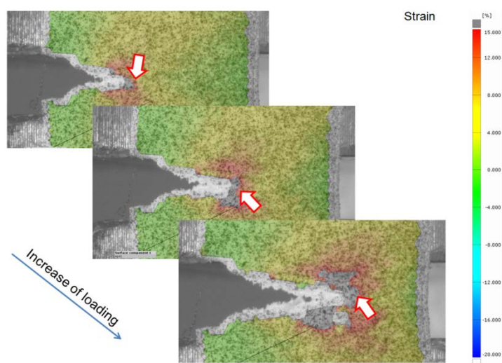
Fig.13. Tracking the crack growth by using the surface strain field (the arrows mark the current crack tip, 15 % strain).
