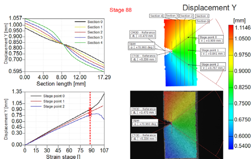
Fig. 9. Report from Aramis system software for SENT specimen.
