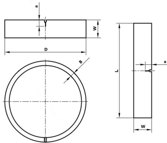
Fig. 2. Drawing with marked dimensions – PRNT and SENT specimen.
