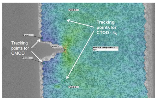
Fig. 10. Strain field obtained by DIC and measurement points for CMOD and CTOD- \delta_5 .
