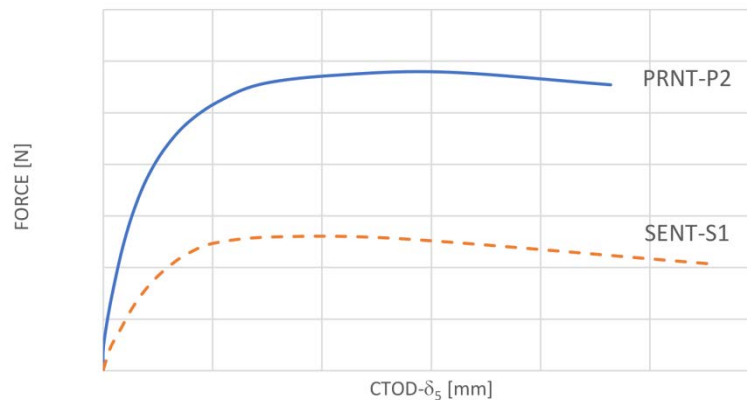
Fig. 12. Dependence of force on CTOD- \delta_5 for a PRNT and a SENT specimen.
