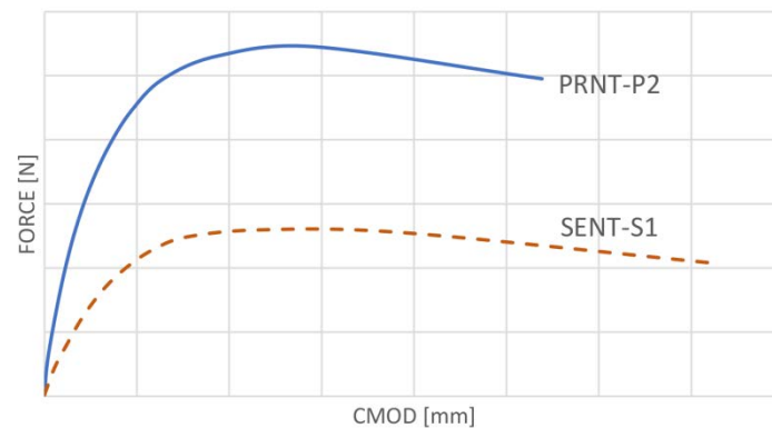
Fig. 11. Dependence of force on CMOD for a PRNT and a SENT specimen.
