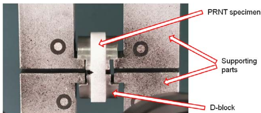
Fig. 5. PRNT specimen and tools for testing.
