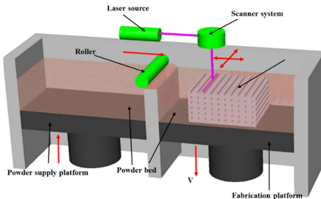
Fig 1. Schematic display of SLS device assembly and working principle [10].
