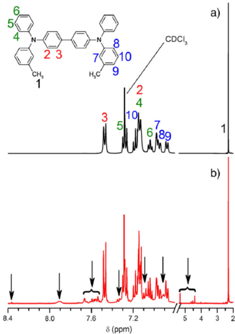
Fig.3.9 1 H NMR spectrum of a dissolved pristine TPD film with the main resonance assigned to protons attached to 10 unique carbon atoms in TPD; see the drawing of TPD molecular structure in the inset. b) The corresponding spectrum of UV irradiated TPD film with additional resonances (indicated by arrows and braces) due to photo-oxidized TPD species.
